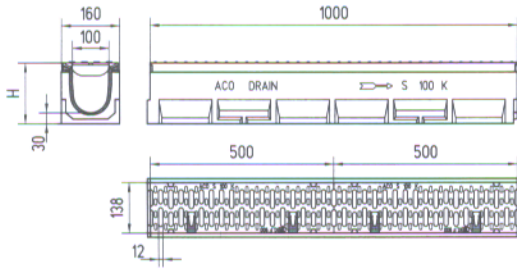
S 100 K, 1.0 m
