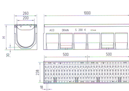
S 200 K, 1.0 m
