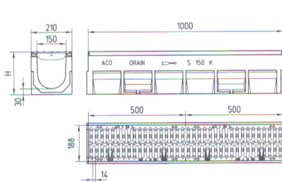
S 150 K, 1.0 m
