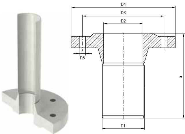
AP connector with flange and spigot
