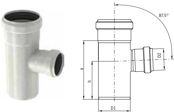
AP single branch reduction 87.5°
