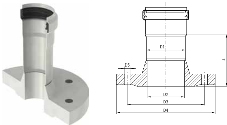
AP connector with socket and flange
