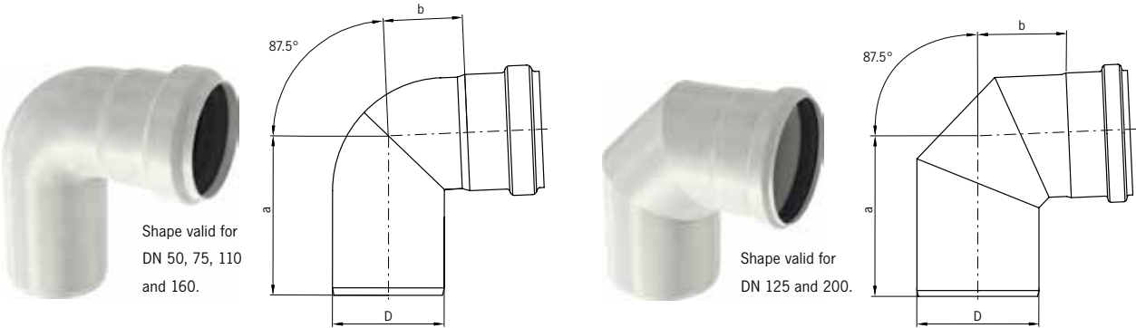
AP bend 87.5°
