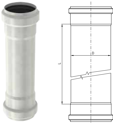
AP double socketed pipe 125 mm
