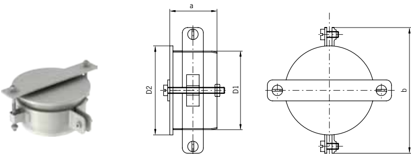
AP socket plug with clamp
