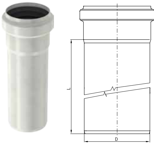
AP socketed pipe 200 mm
