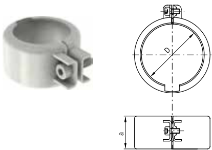
AP socket clamp
