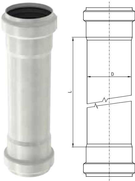
AP double socketed pipe 75 mm
