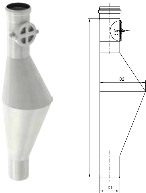
AP rat-stop pipe
