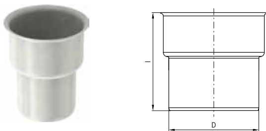
AP connector cast iron spigot → ACO PIPE® socket
