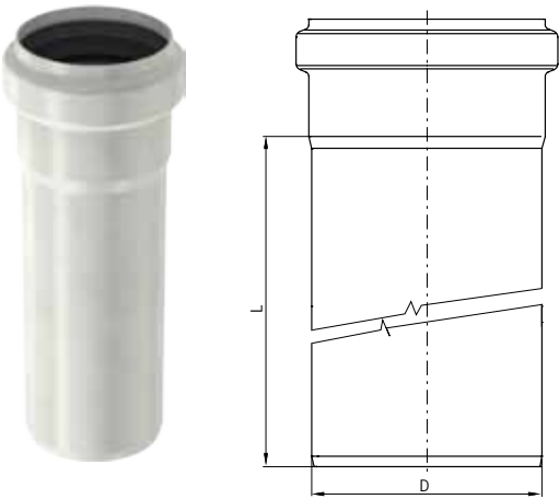
AP socketed pipe 160 mm
