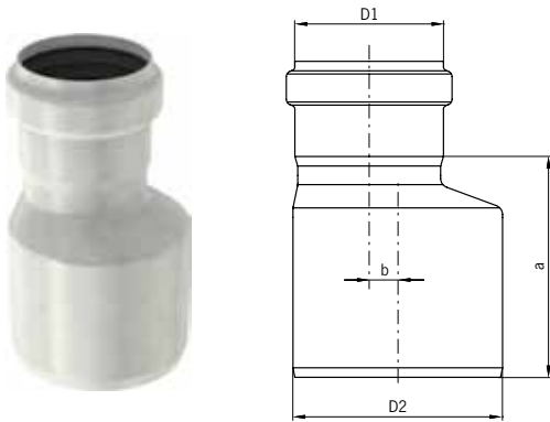
AP eccentric increaser coupling
